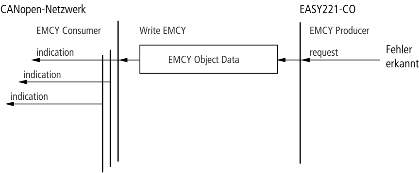
Abbildung 24: Emergency Object Protocol
