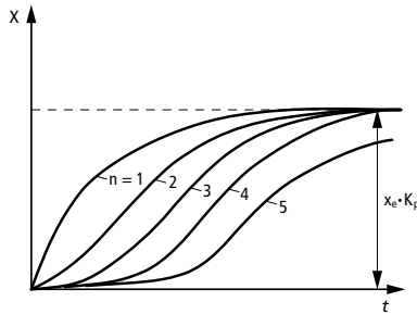
Figure 16: The transition behaviour of PTn gates of various orders (PT1 to PT5)
