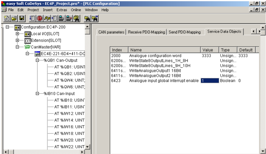
Figure 23: Setting “Analogue input global interrupt enable” to “1” to enable the analog inputs.
