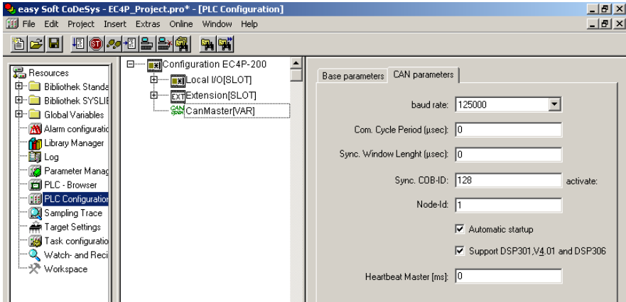
Figure 15: Setting the baud rate and the CAN address (Node-Id) of the CAN master
