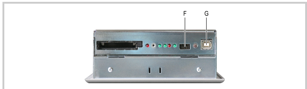
Abb. 11 Interfaces on the service side of the BAS, CAN and MPI devices (figure shows service side of BAS, CAN and MPI devices)
