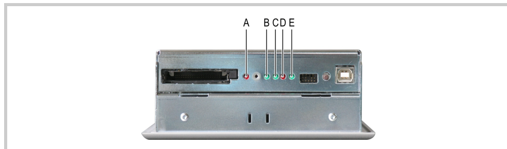
Abb. 7 Indication elements on the service side
