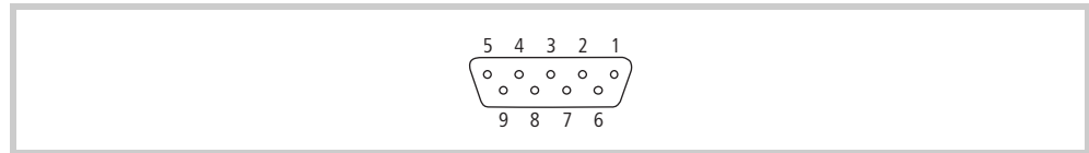
Abb. 23 RS485 interface (9-pin, D-Sub, female, UNC)
