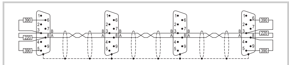
Abb. 22 Bus segment with four bus stations
