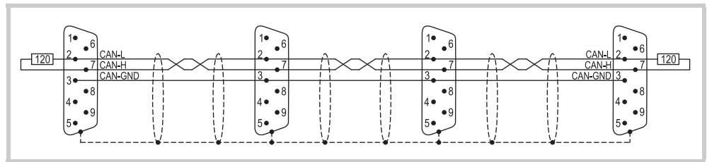
Fig. 13 Bus segment with four bus stations
