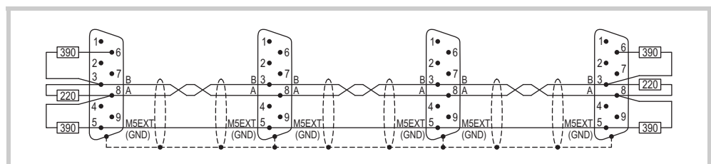
Fig. 15 Bus segment with four bus stations
