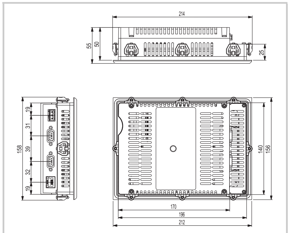
Fig. 23 Mechanical dimensions in mm
