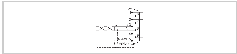
Fig. 16 Alternative termination (only for XV200, MK2)
