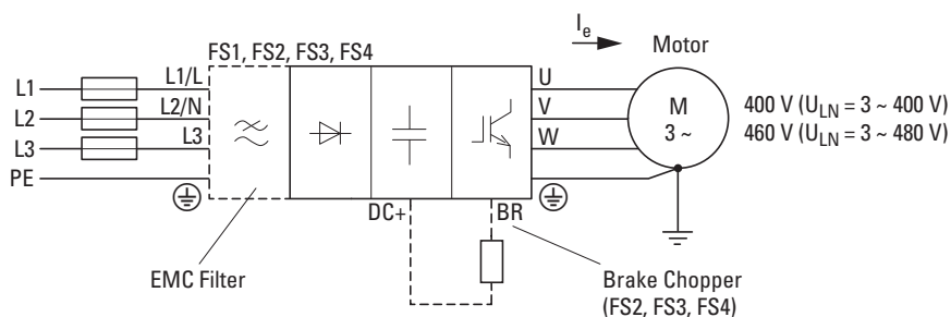
Figura 11: DC1-34...
