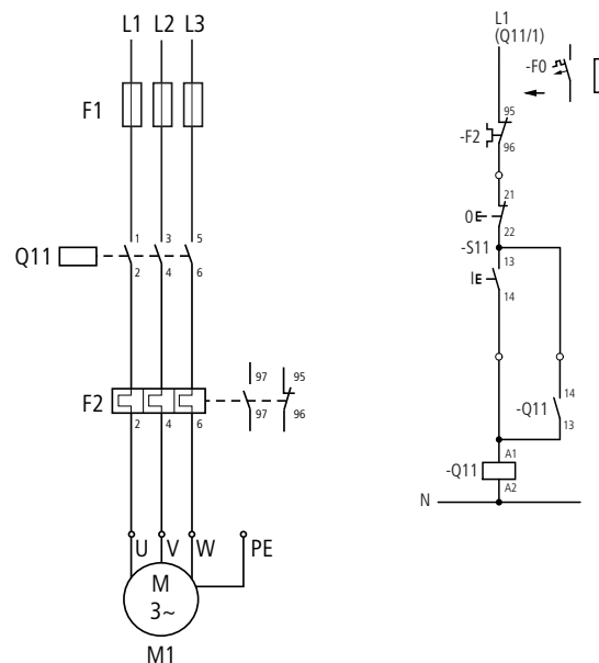
Figure 6: Circuit prevents automatic restart
